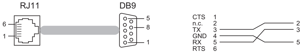
Figure 17: Pin assignment of the V.24 interface and wiring to the DB9 connector
