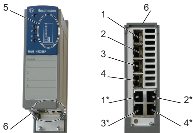
Figure 7: Port assignment
