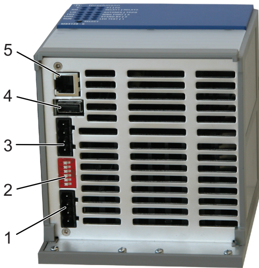
Figure 4: Connections on the bottom of the basic module 1 – Terminal block (Power 2) 2 – DIP switch 3 – Terminal block (Power 1) 4 – USB port 5 – V.24 port
