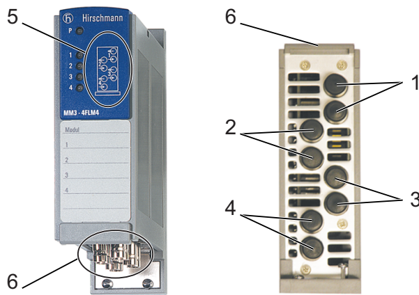
Figure 6: Port assignment
