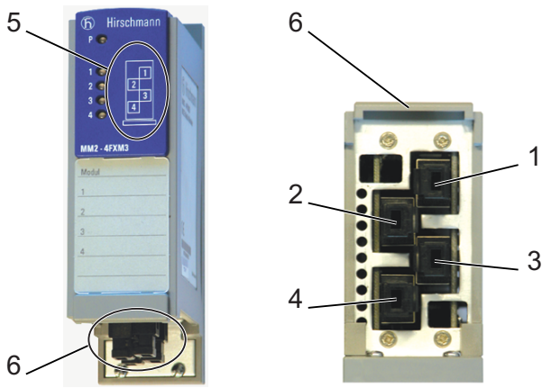
Figure 5: Port assignment
