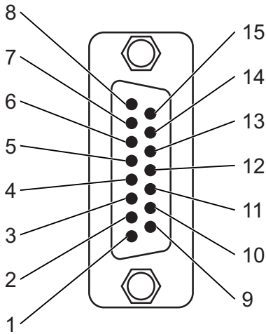
Figure 14: Pin assignment of an AUI interface
