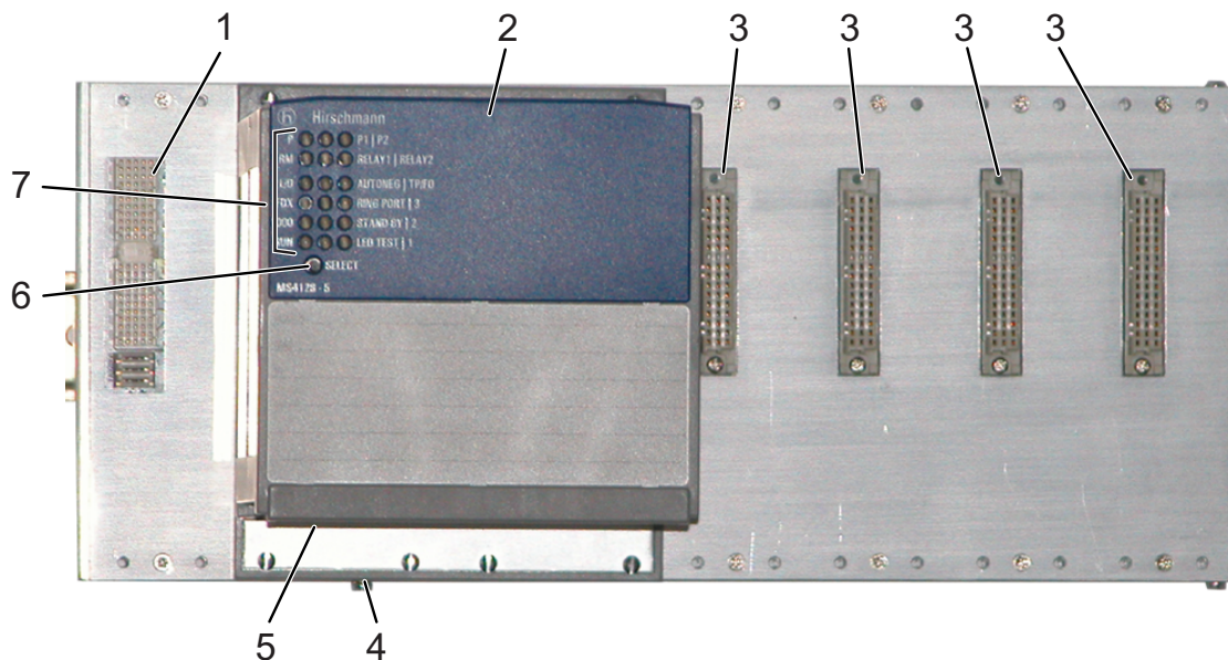
Figure 2: Front of the basic module
